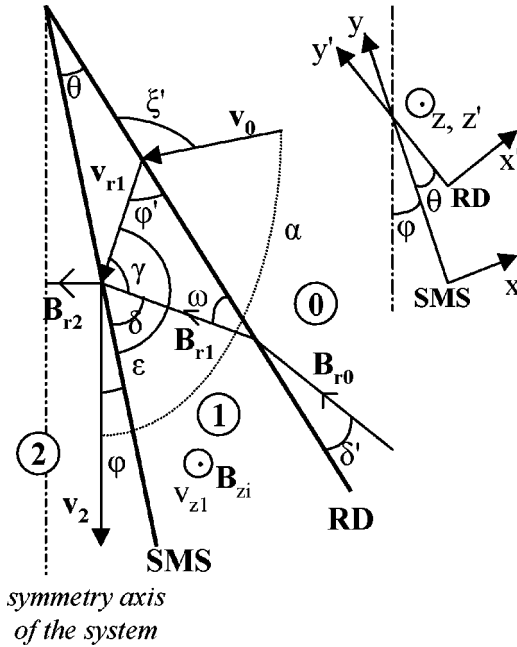
FIG. 1. The geometry of the system of discontinuities in the 2\frac{1}{2} D symmetrical reconnection problem, depicted in one quadrant. The slow-mode shock (SMS) is inclined to the symmetry axis (dash-dotted line) at the angle \phi . The angle between the rotational discontinuity (RD) and the SMS is denoted as \vartheta . The quantities in the inflow, intermediate, and outflow regions are designated by subscripts “0,” “1,” and “2,” respectively. The xy -plane components of the magnetic field \vec{B} and the flow velocity \vec{v} are denoted by the subscript “ r .” The direction of the z component of \vec{B} and \vec{v} is also indicated. The incidence angle of the inflow is denoted as \alpha . The y' axis of the “primed” frame of reference is aligned with the RD, while the y axis of the “nonprimed” coordinate system lies aligned with the SMS, as shown upper right.
